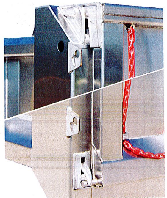
Pictured is a close view of the tarp friendly stainless upper hardware and the stainless lower latching hardware standard on the 553U
